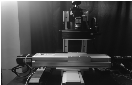
图 11 COB LED 显示模组墨色采集平台(包含相机、光源) Fig.11 Platform of COB LED display module ink collection (including camera and light source)
